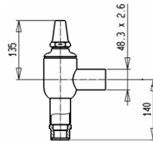
EA40-SS/G1"-I
