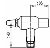
EA40-SS/G1"-II
